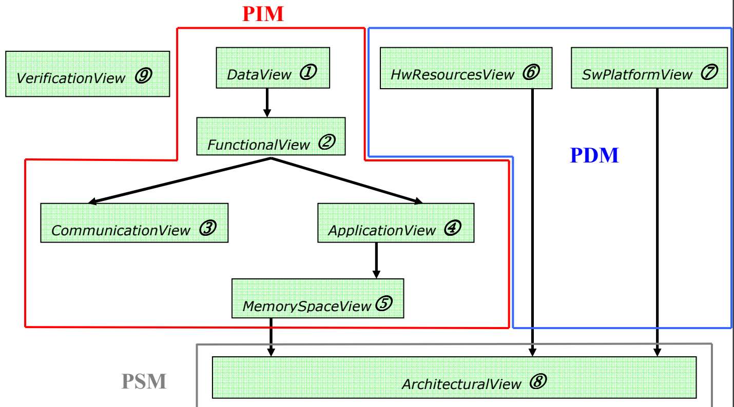
Figure 1 UML/MARTE view modelling activity
